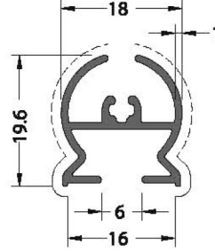
connectionsashprofile arakanatprofil
