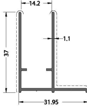
wall connection profile duvardikmesi
