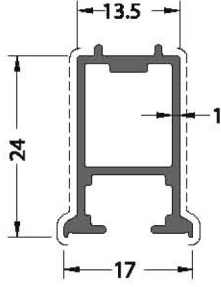
vertical frame profile arkapano
